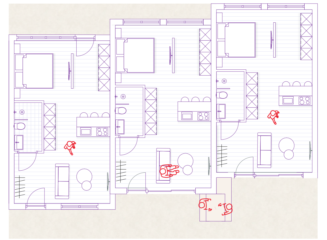
Woningen expats 1:100
