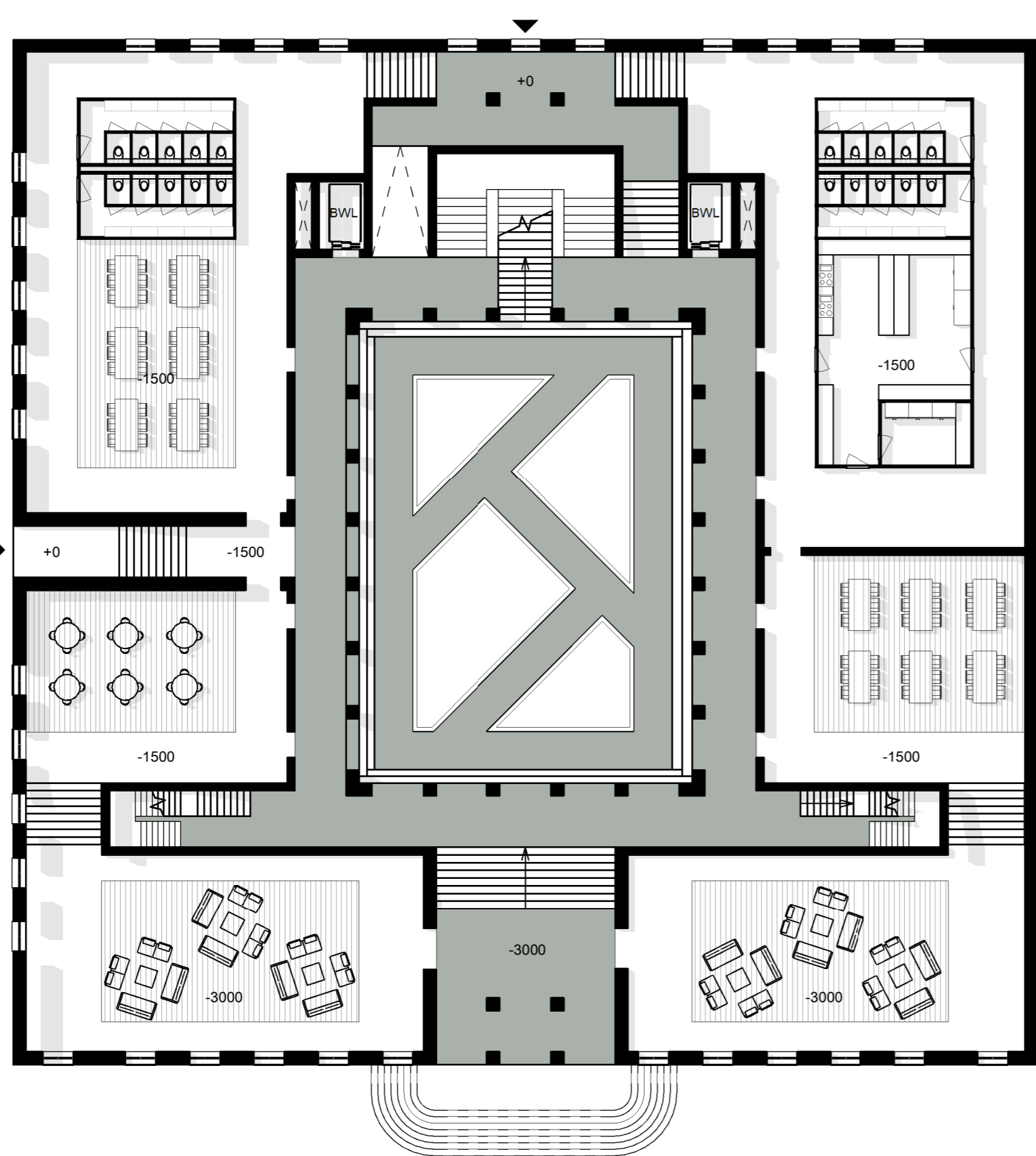
BEGANE GROND 1:200
