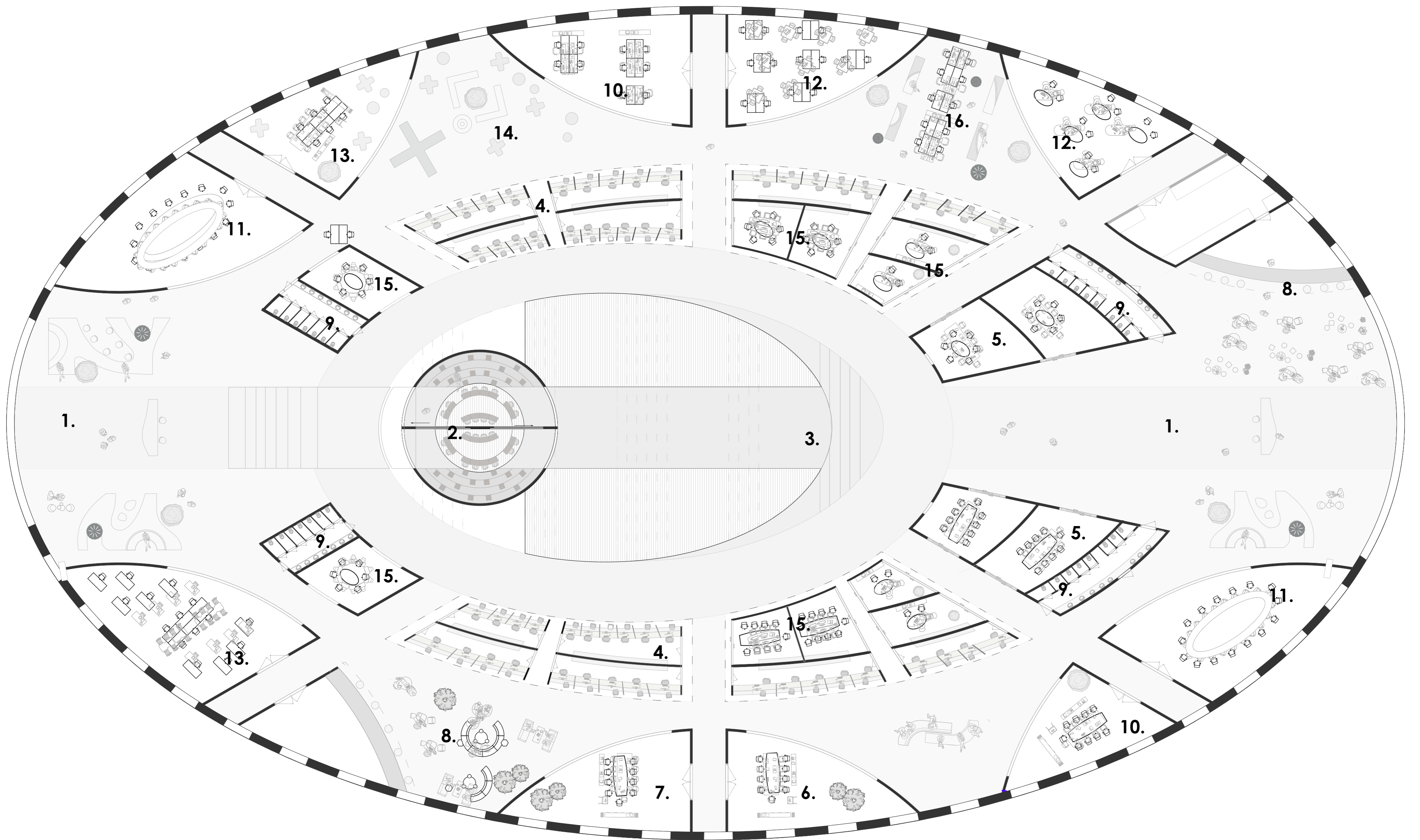
Ground floor Scale: 1:250
