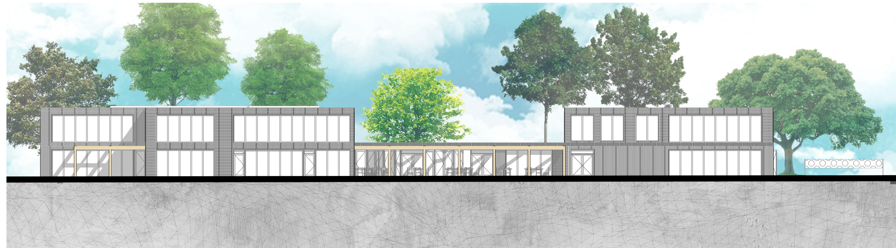
West elevation 1:200
