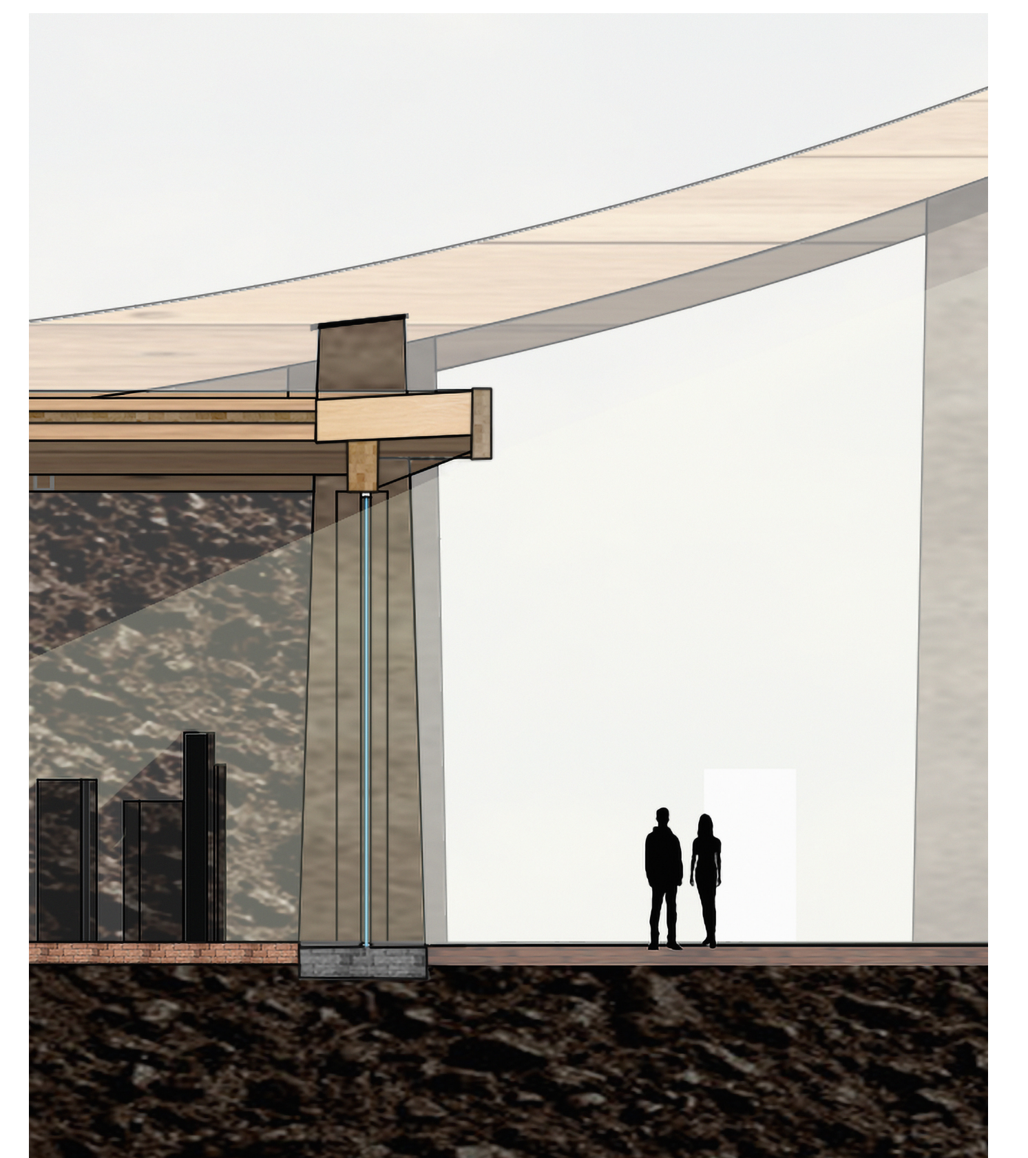
Section 1:50
