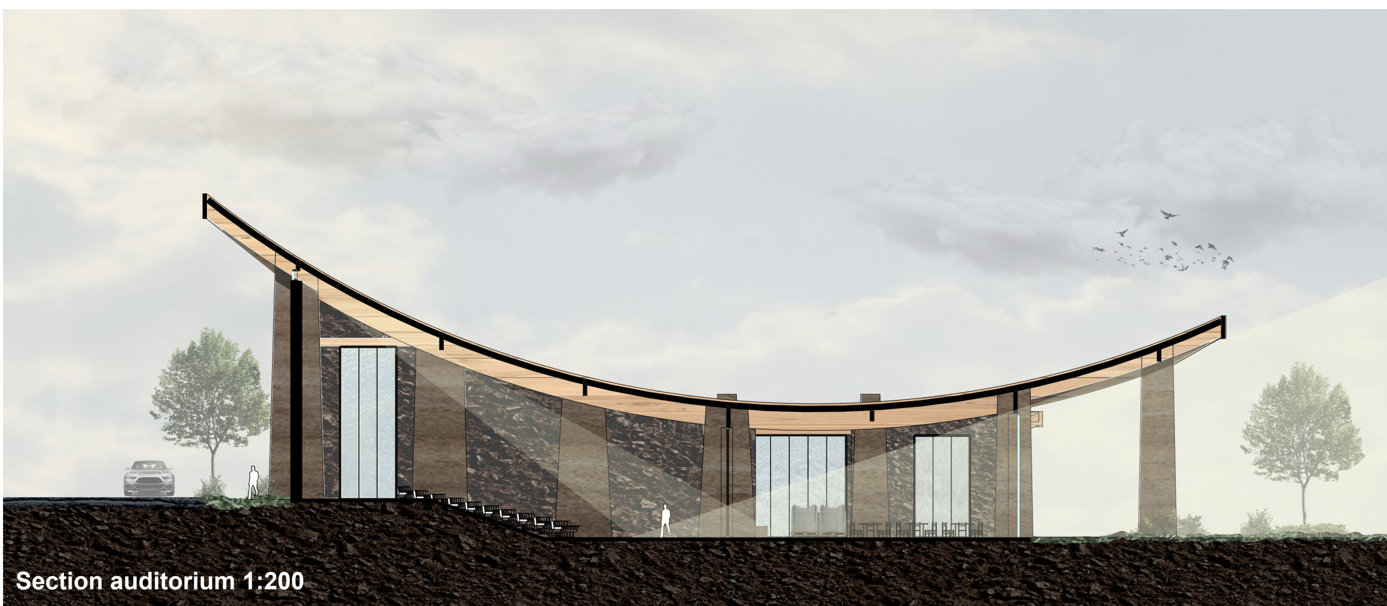
Section auditorium 1:200
