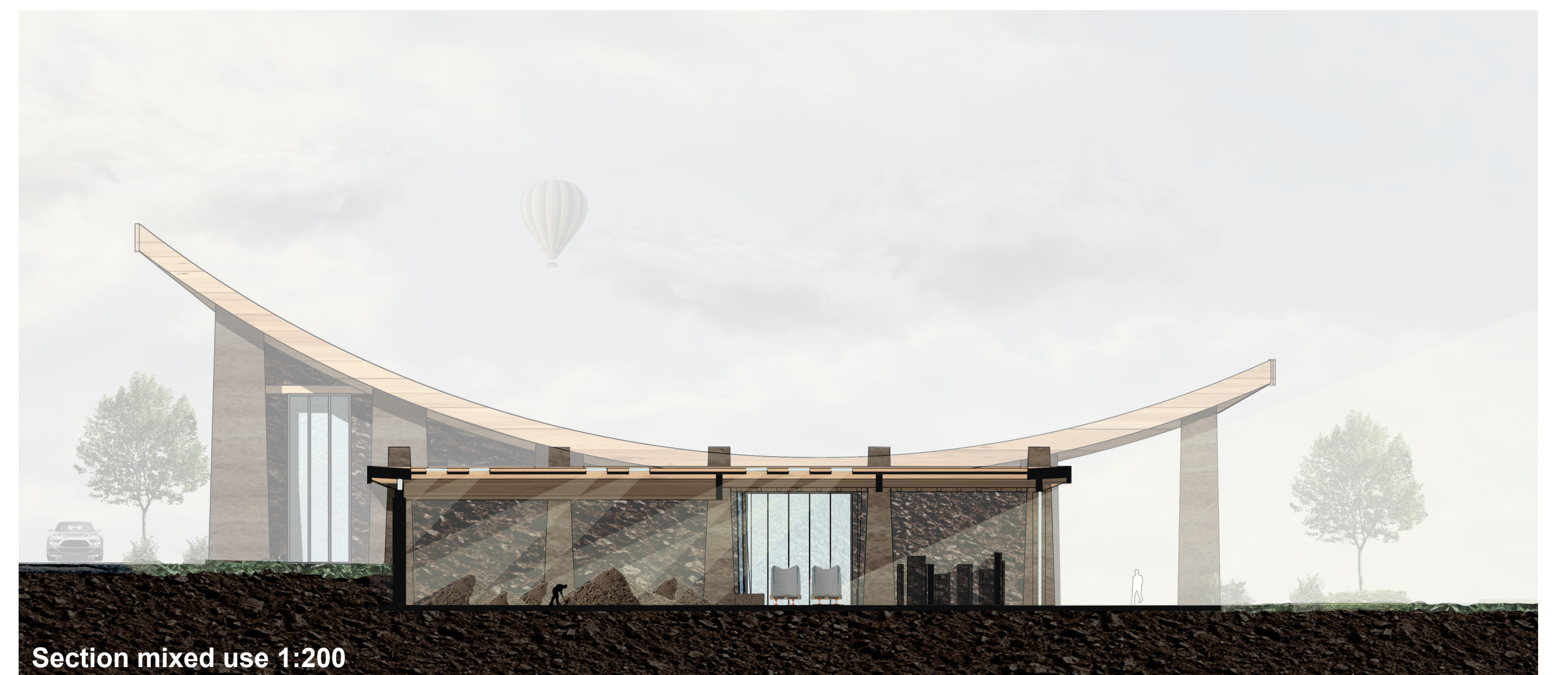
Section mixed use 1:200
