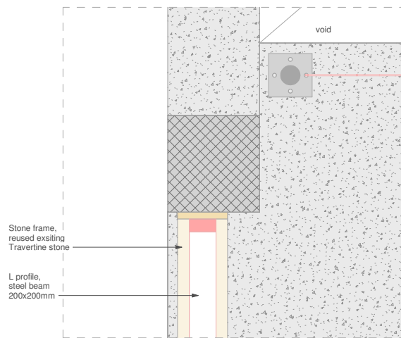
Detail 2_H
