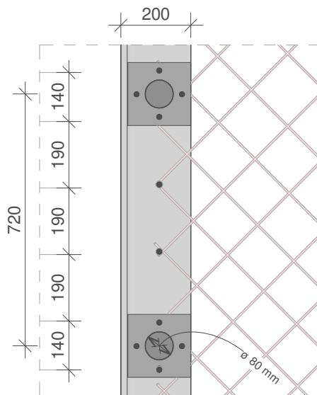
Detail 3_H
