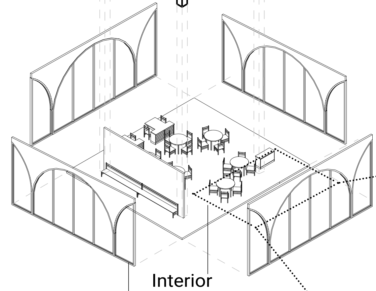
Exploded view: classroom
