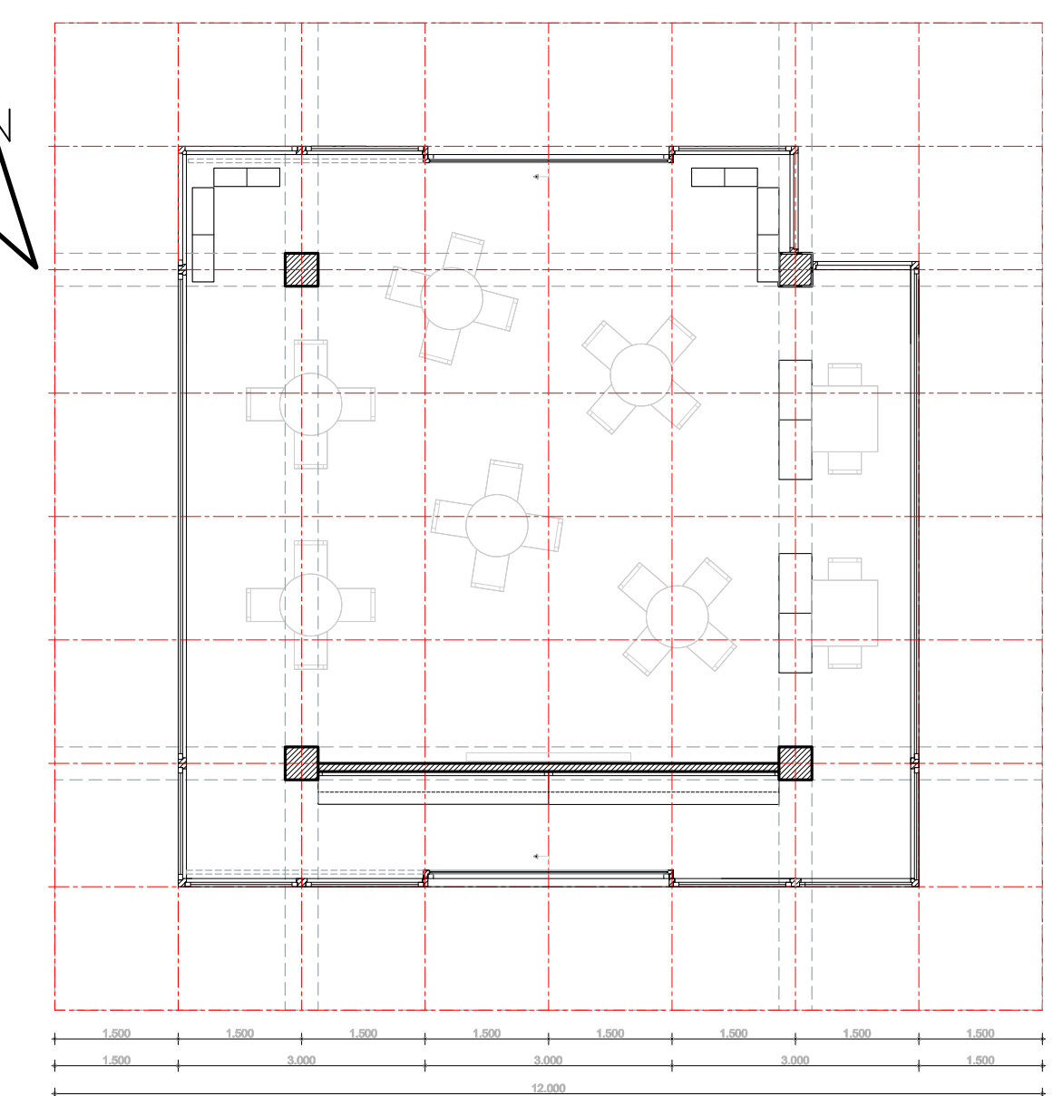
Floorplan: classroom
