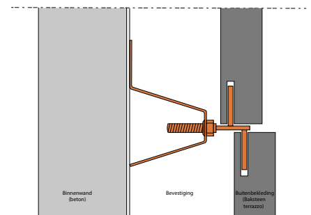
Bevestigings detail
