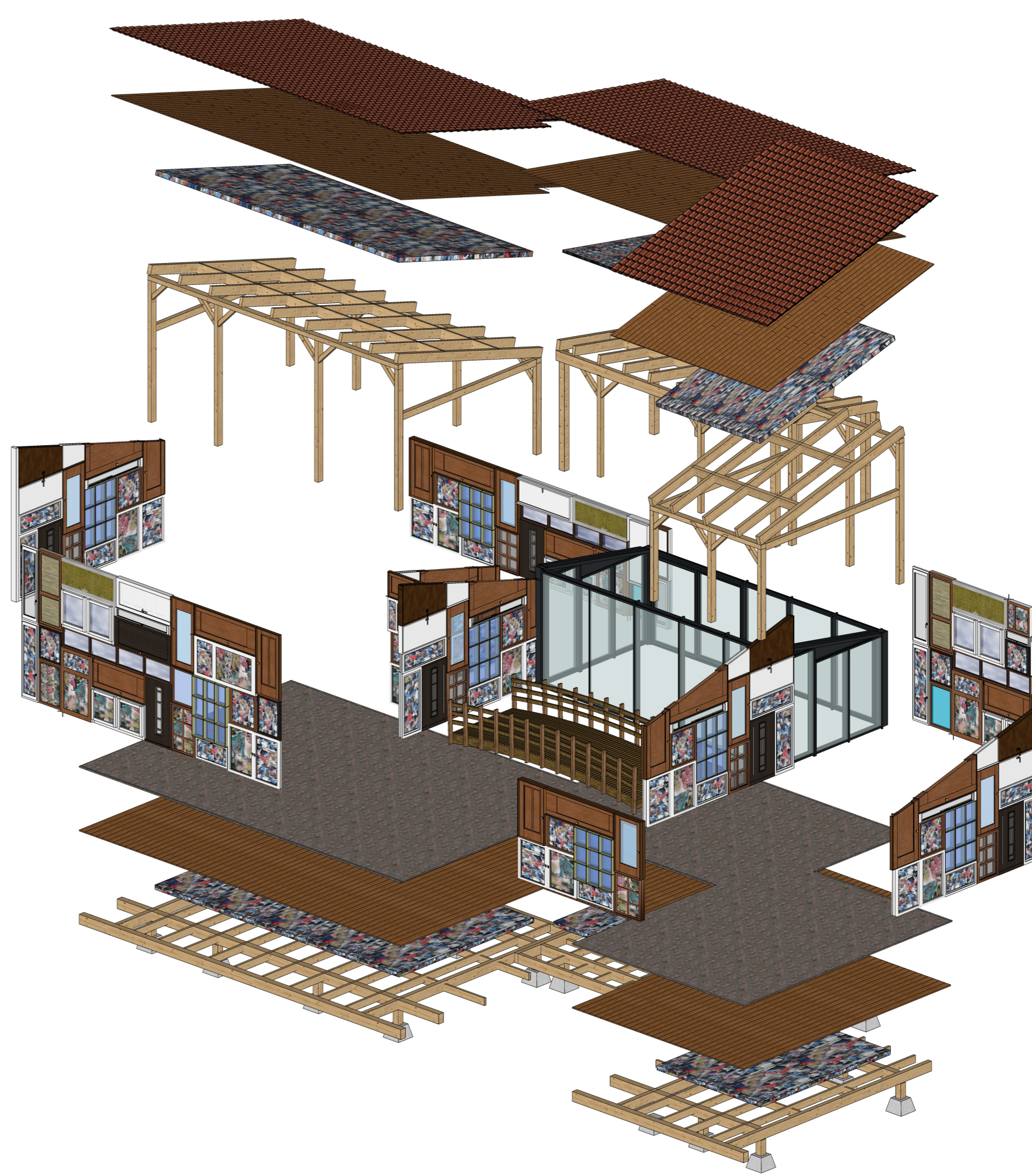
IMPRESSIE: EXPLOAD VIEW
