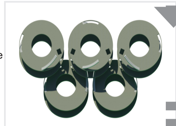
Diagram 2, Routing
