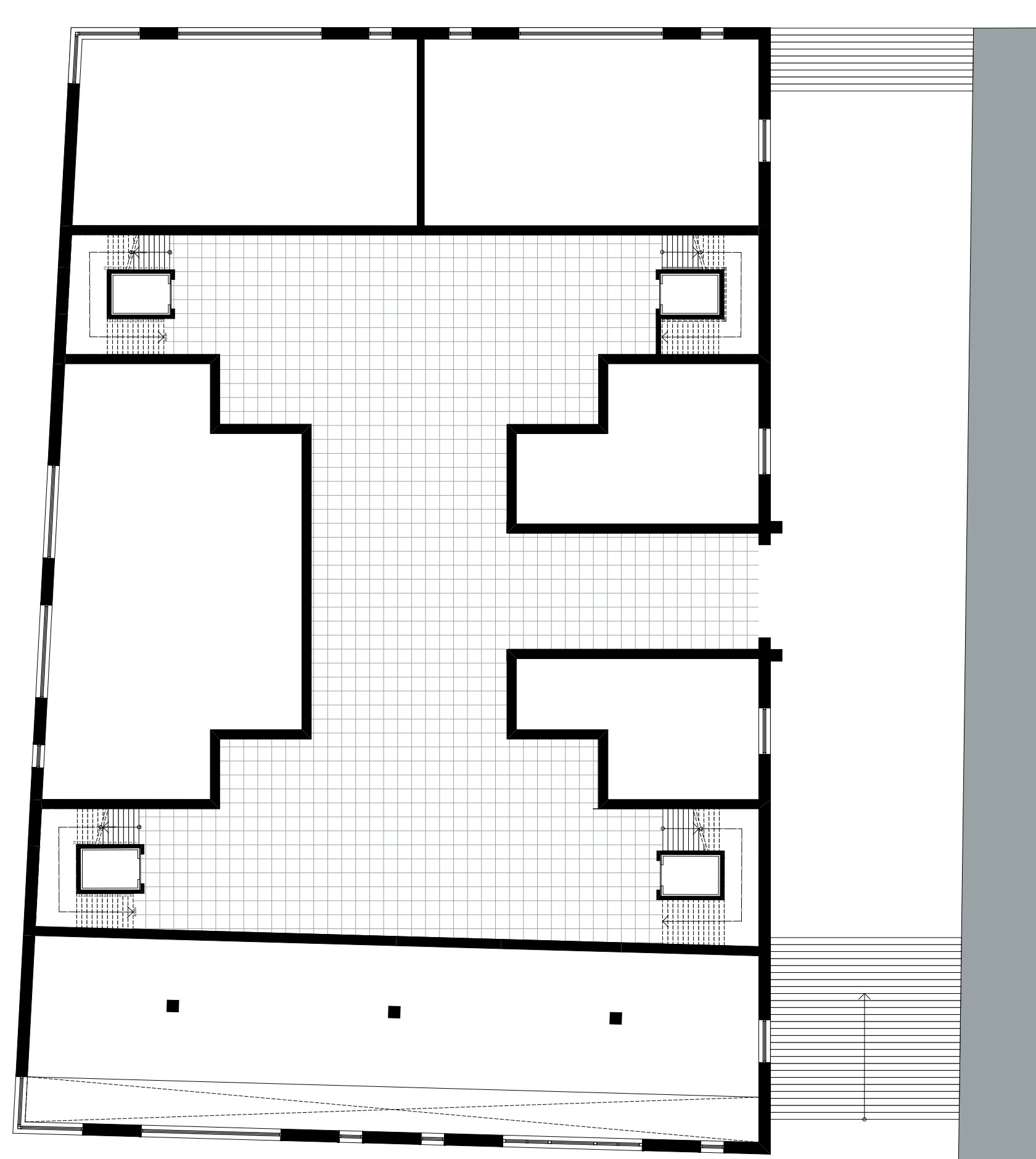
First floor | 1:200
