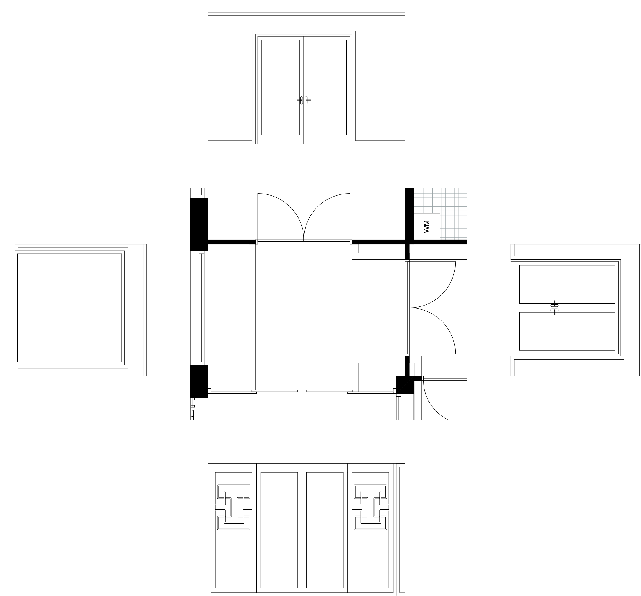
Wall elevations | 1:50
