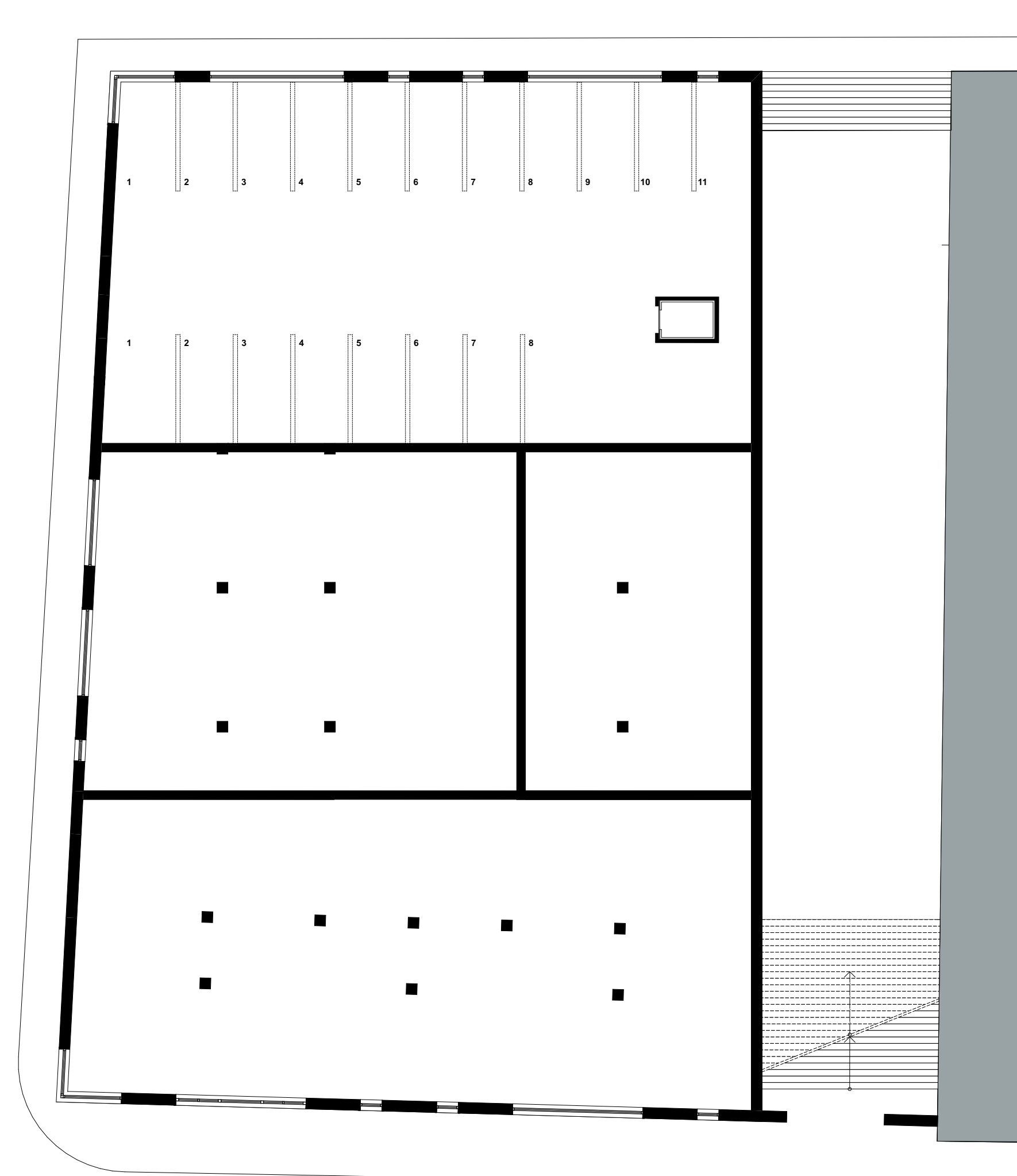
Ground floor | 1:200
