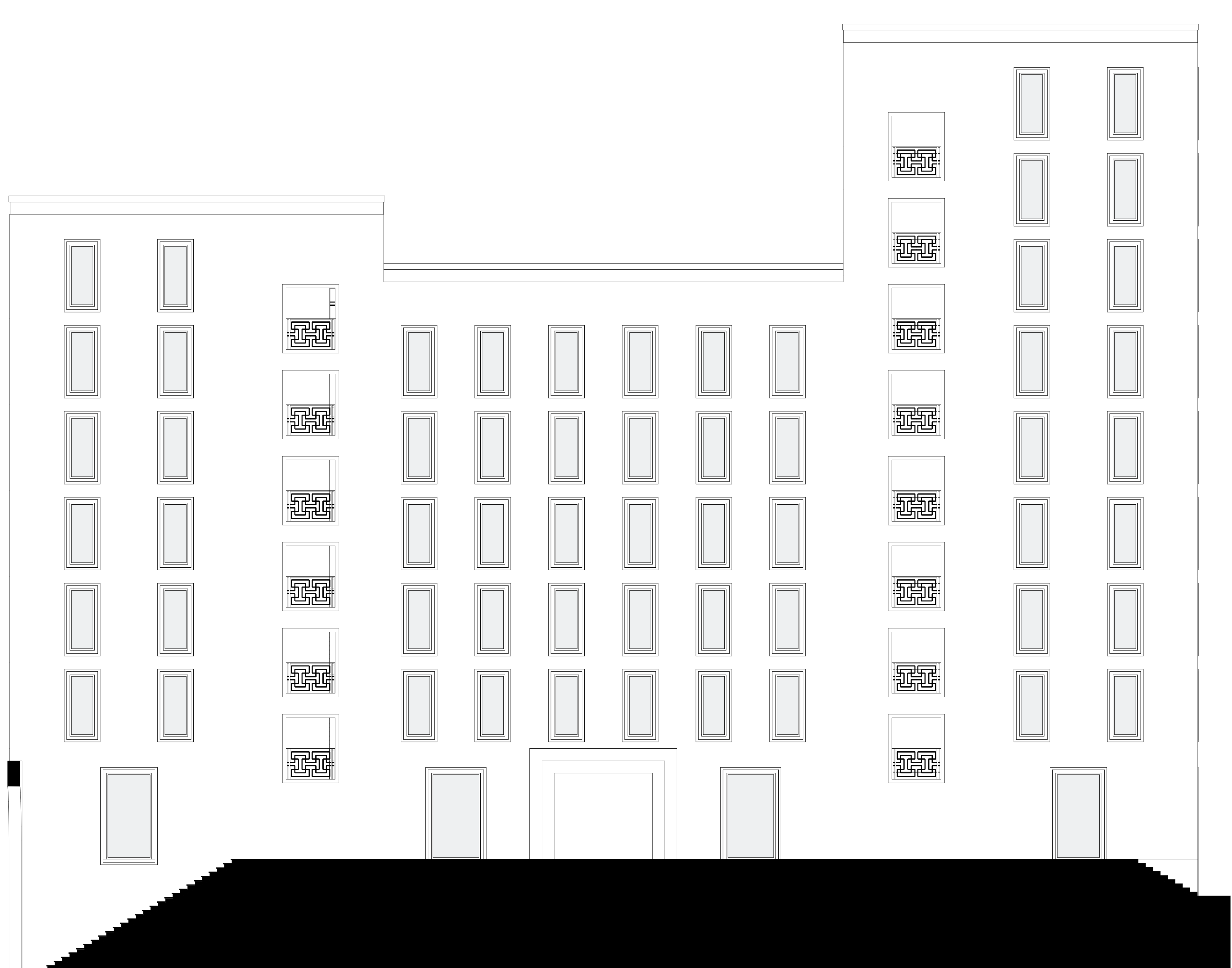
North | 1:100
