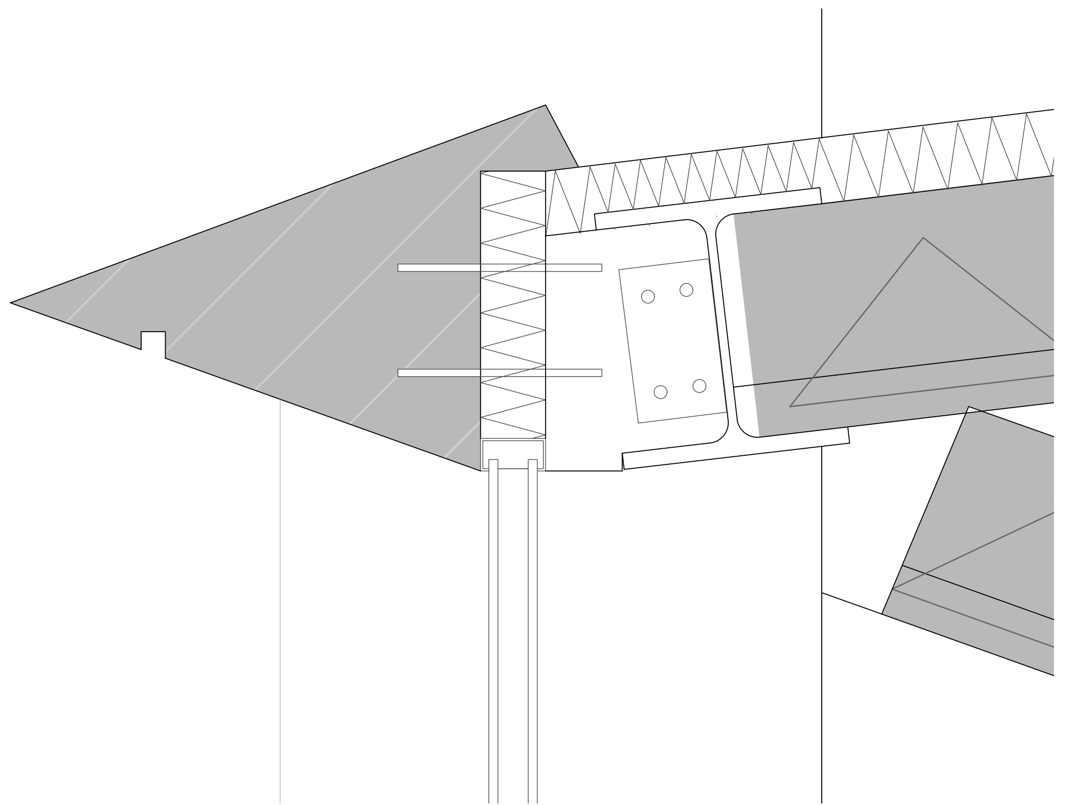
Detail 2 1:5
