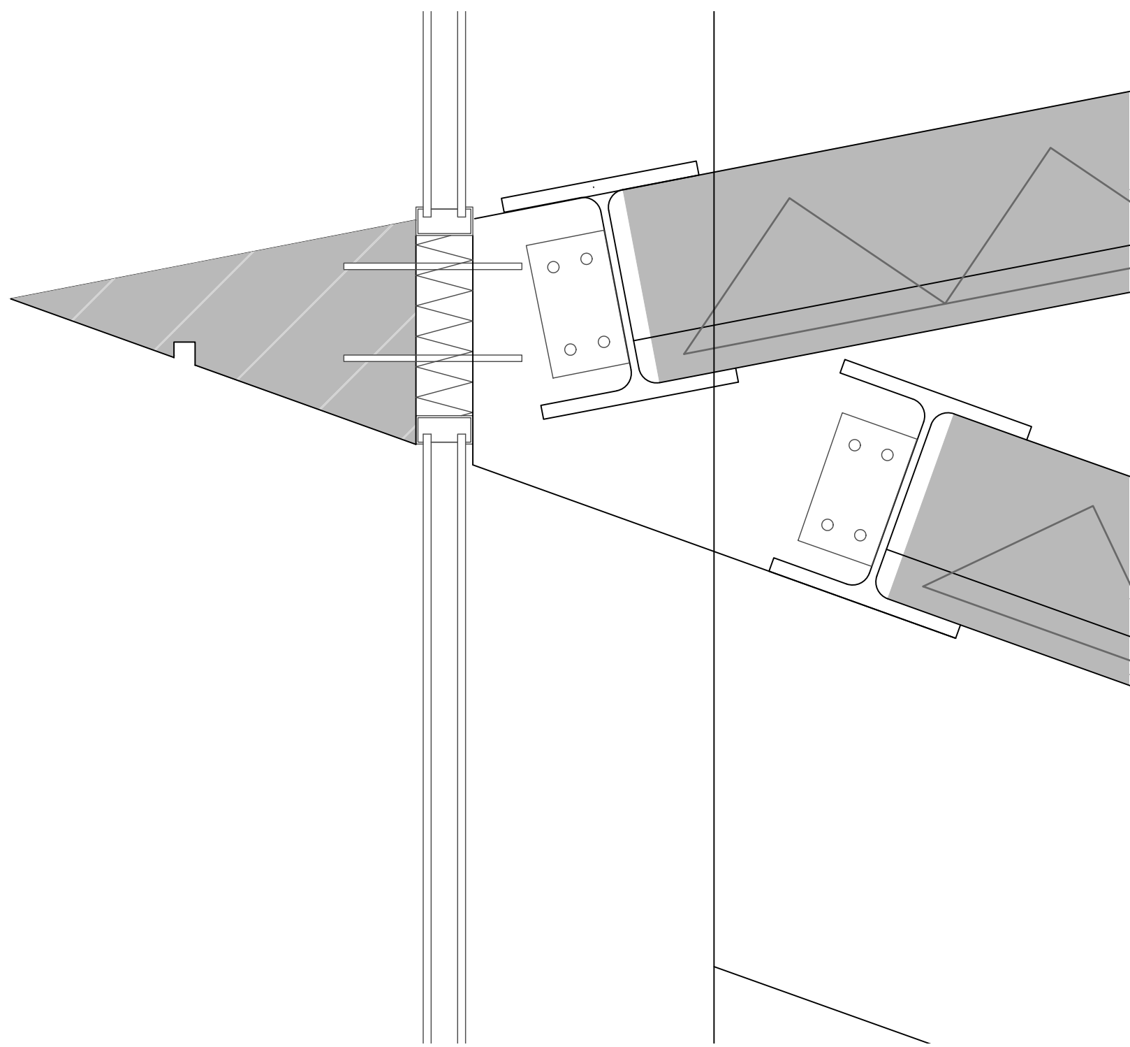
Detail 1 1:5
