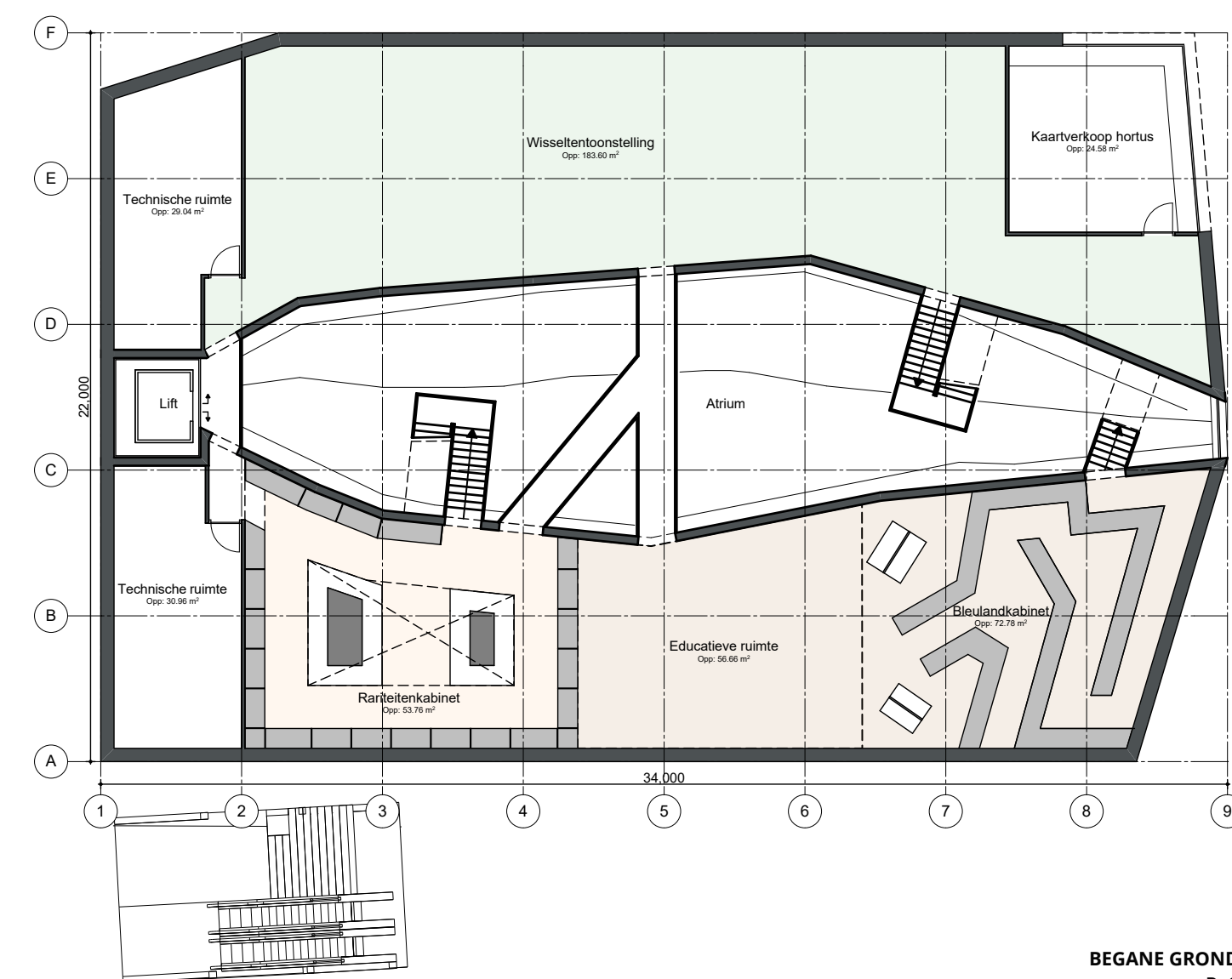
BEGANE GROND P+0
