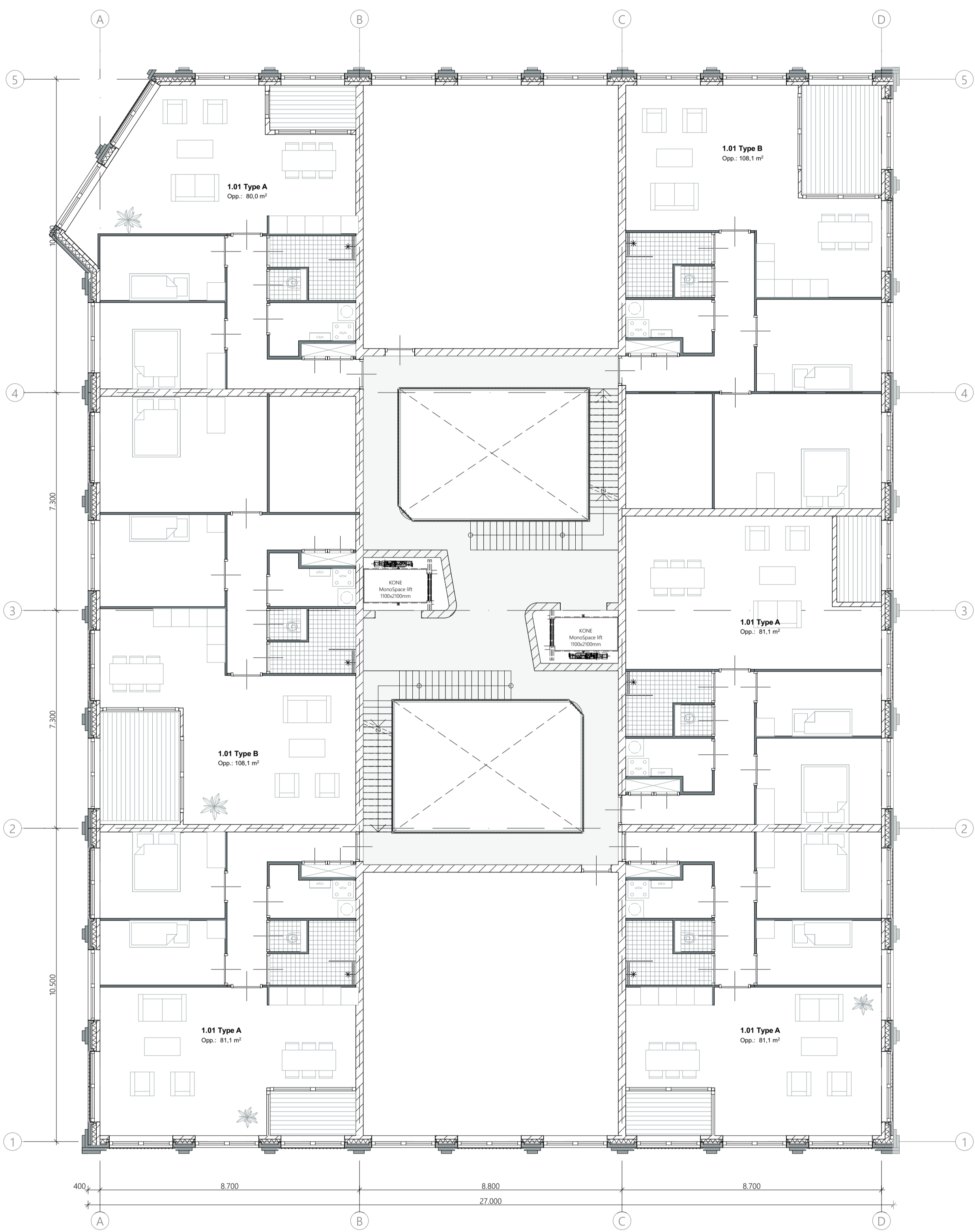
1ST FLOOR
