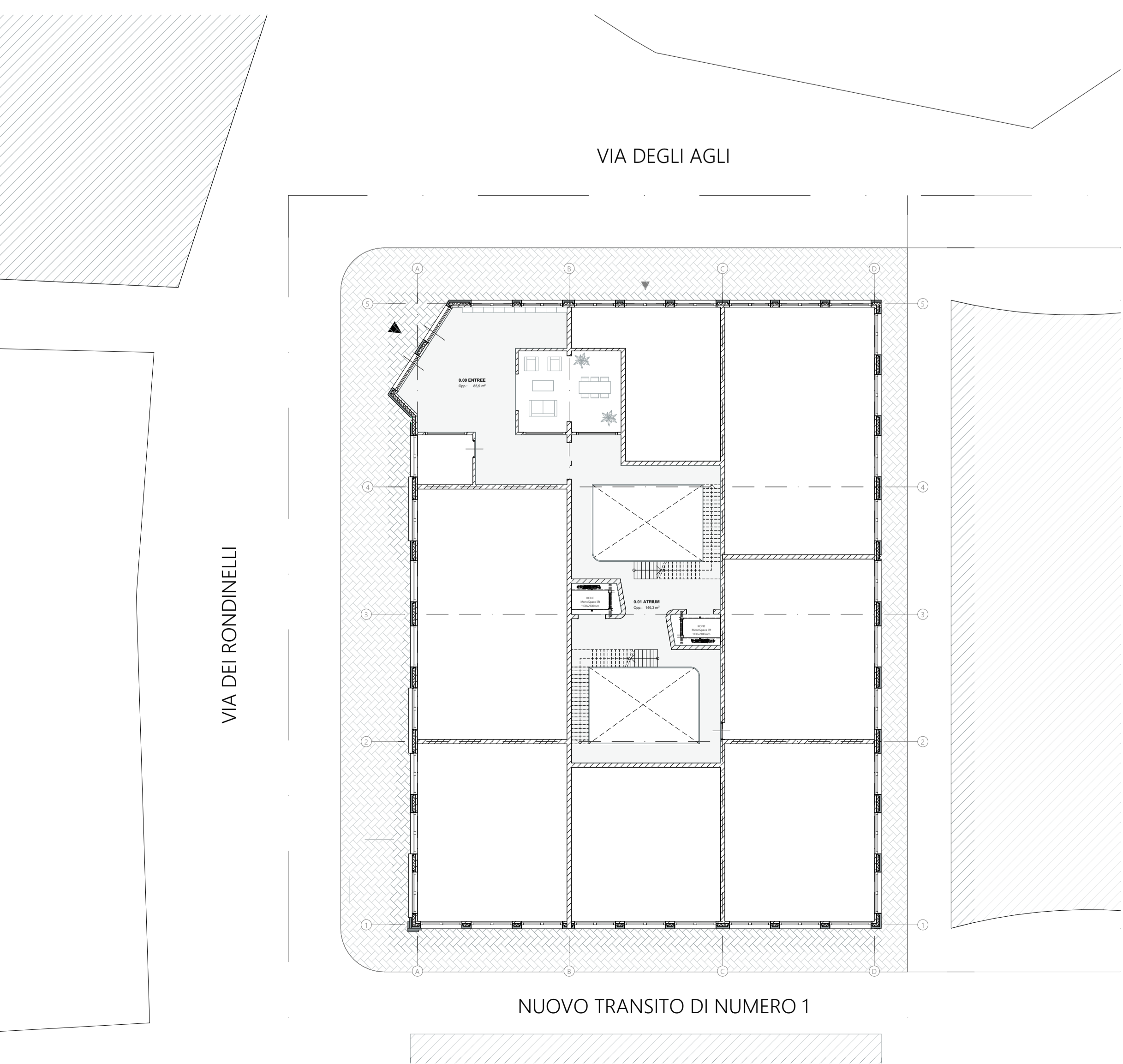
SITUATION, GROUND FLOOR
