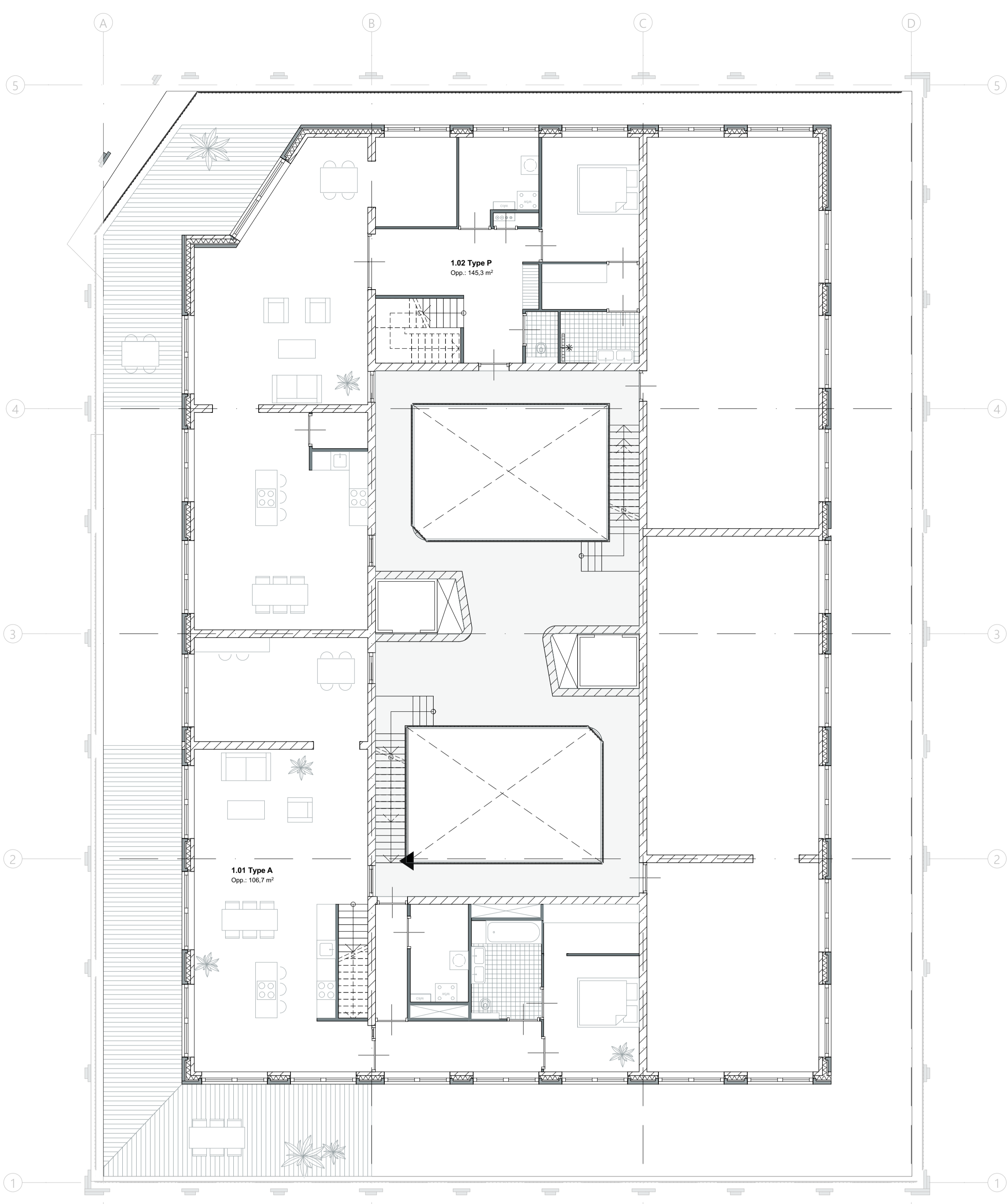
4TH FLOOR
