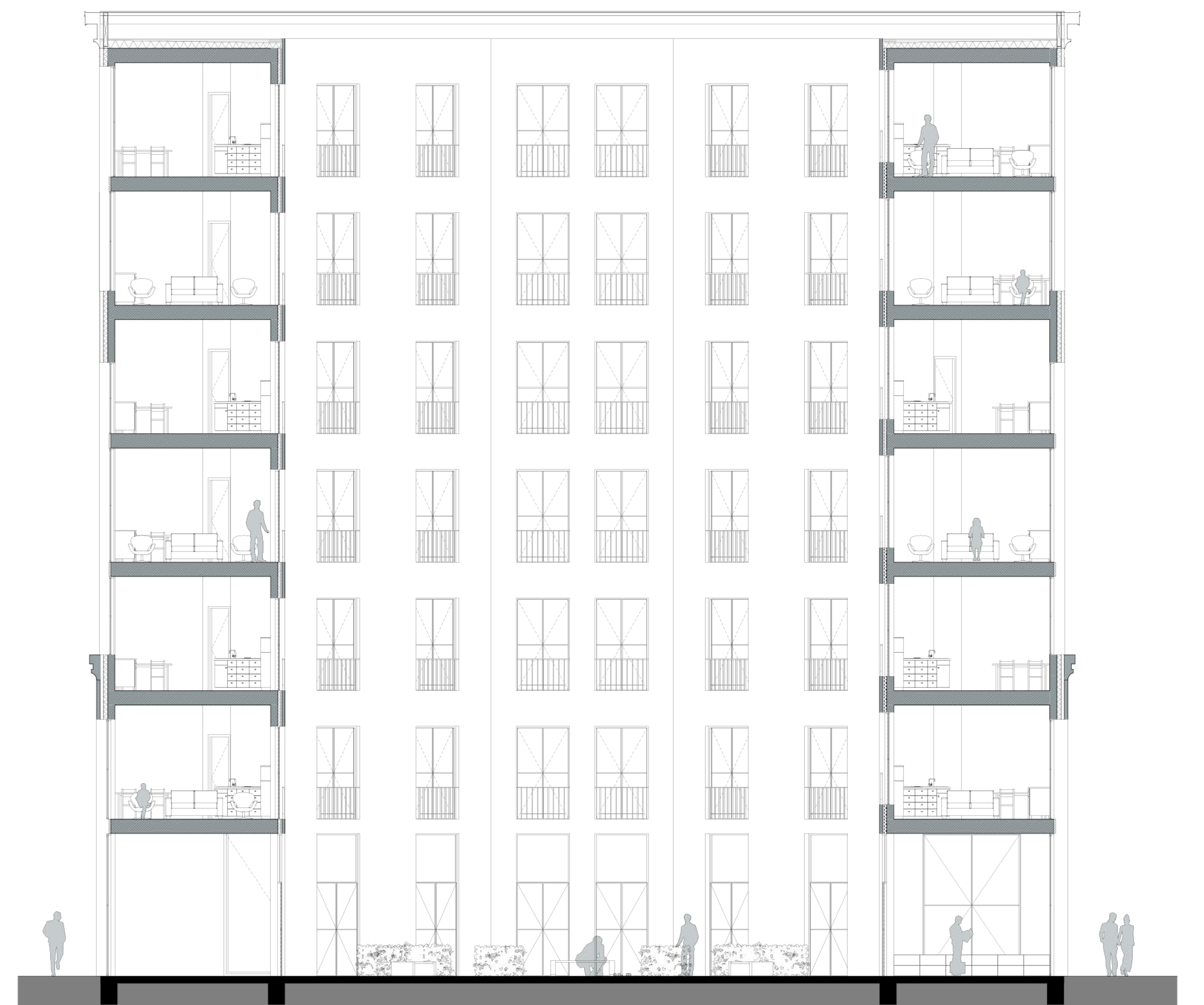
Section
