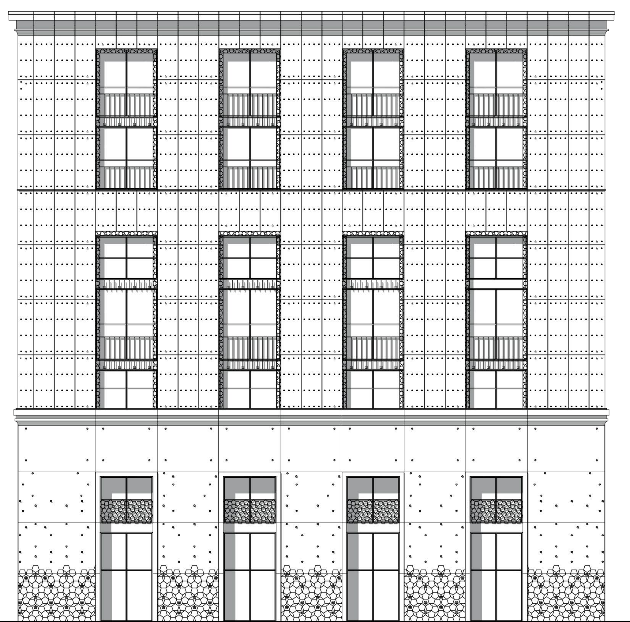
North/South Elevation
