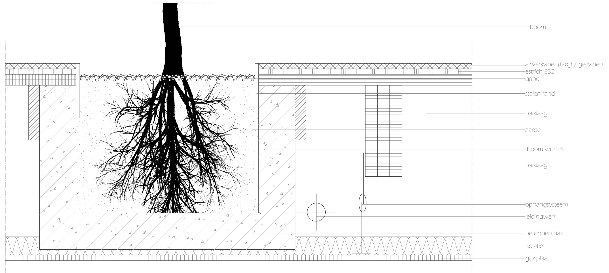
Detail 1:10
