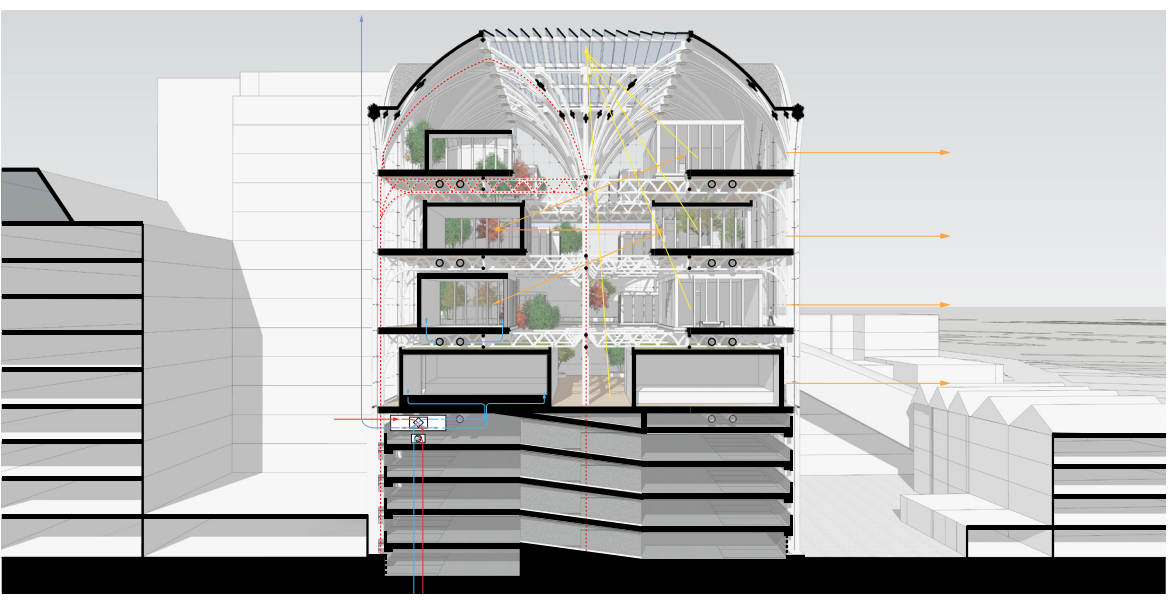
General section
