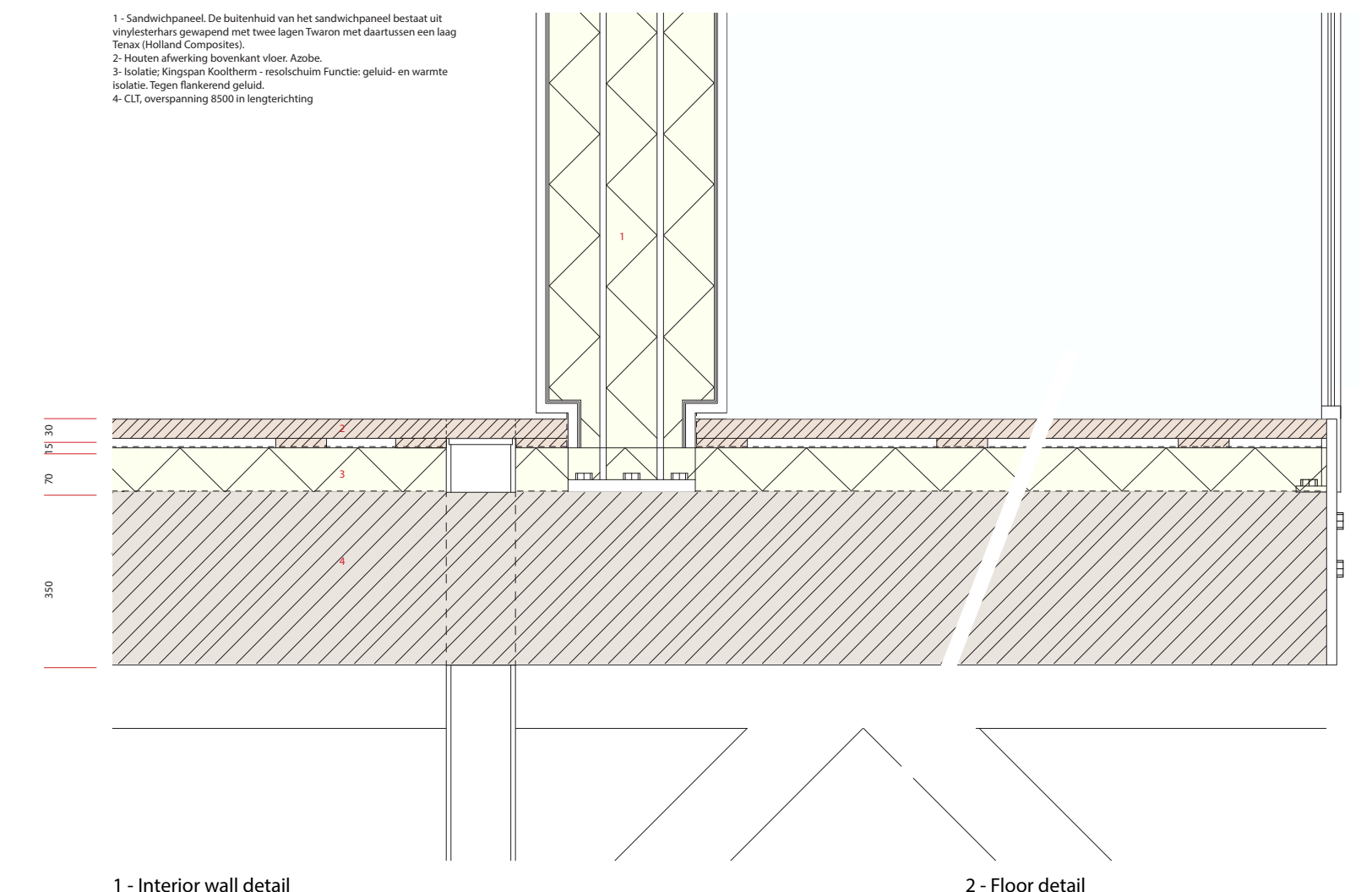
1 - Interior wall detail
