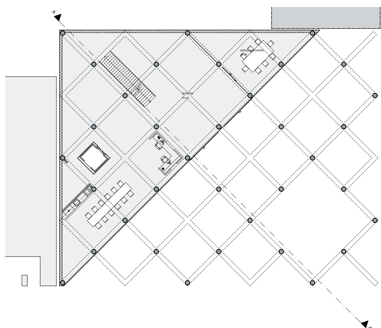
begane grond, 1:200
