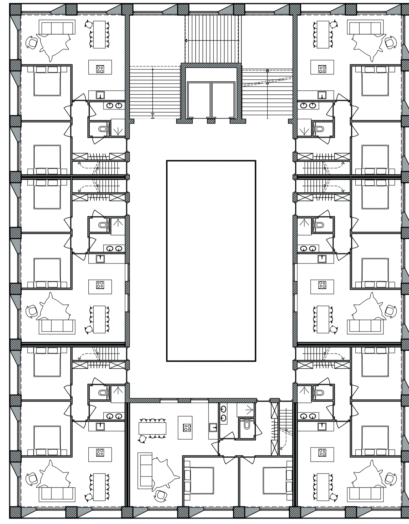
1st Floor, 80sqm apartments
