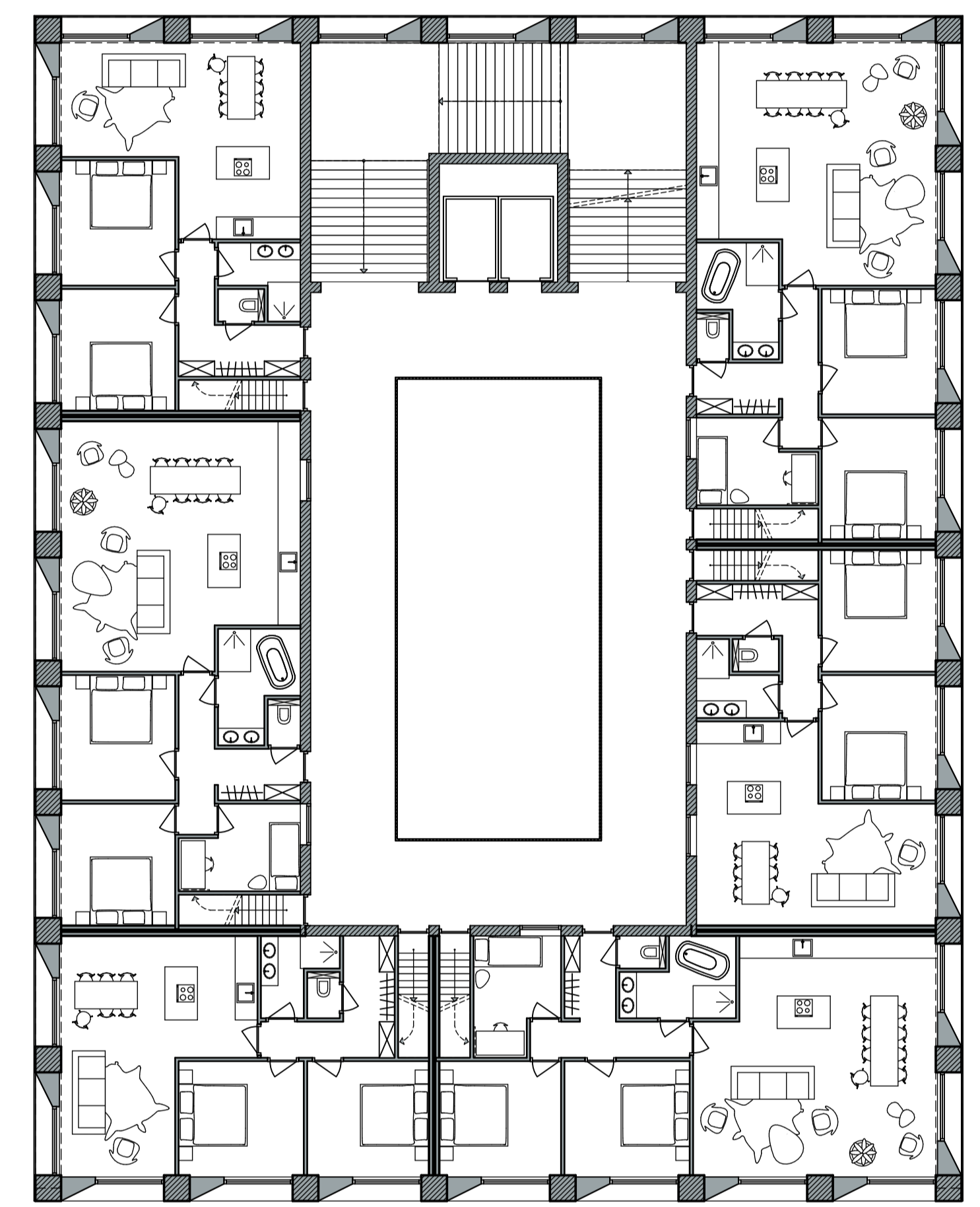
3rd Floor, 80 and 100sqm apartments
