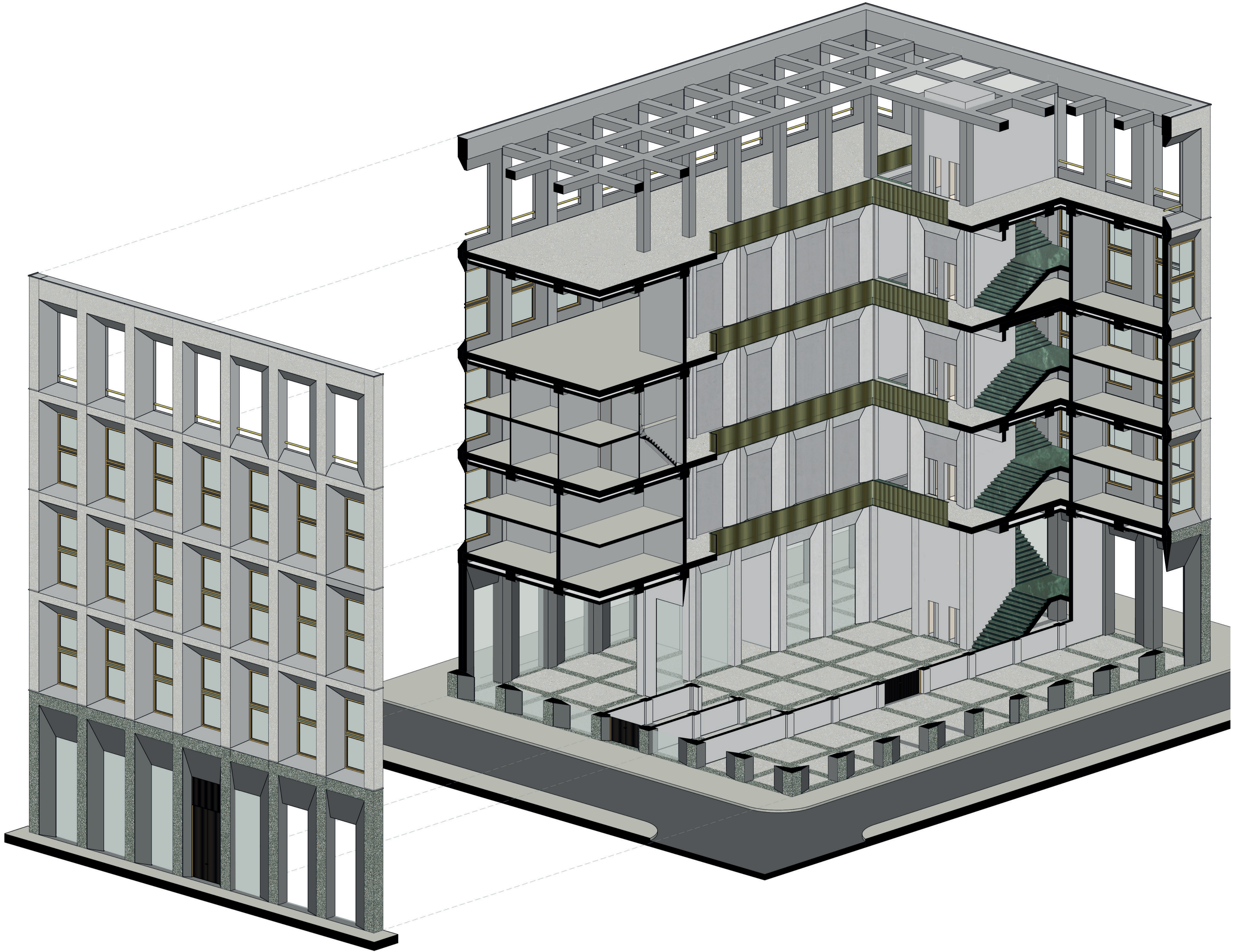
Axonometric Projection
